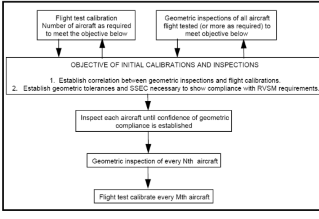
Figure A-5. Process for Showing Initial and Continued Compliance of Airframe Static Pressure System
